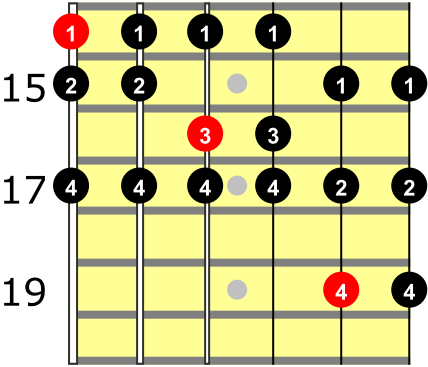
F# LOCRIAN
