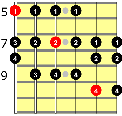
A DORIAN
