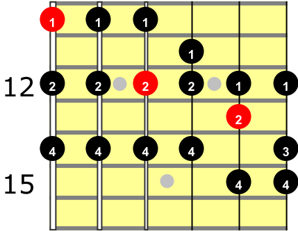
D MIXOLYDIAN
