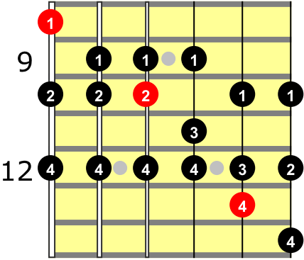
C LYDIAN
